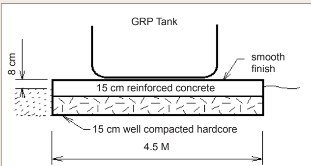
Simple foundation requirements
